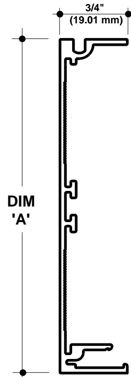
TYPICAL SECTION Perimeter Trim NO SCALE
